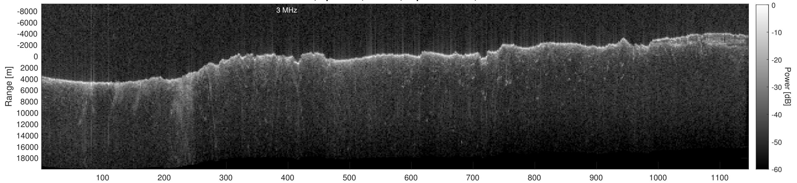
Orbit 15332, Depth-Corrected Cluttergram
