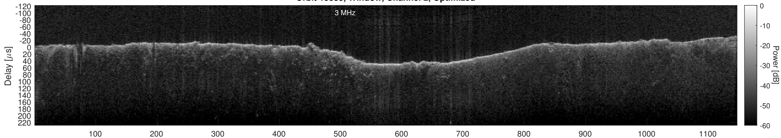
Orbit 15333, Cluttergram
