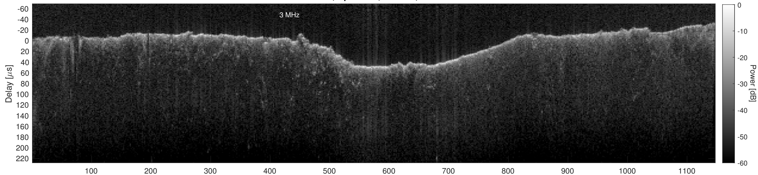
Orbit 15333, Cluttergram
