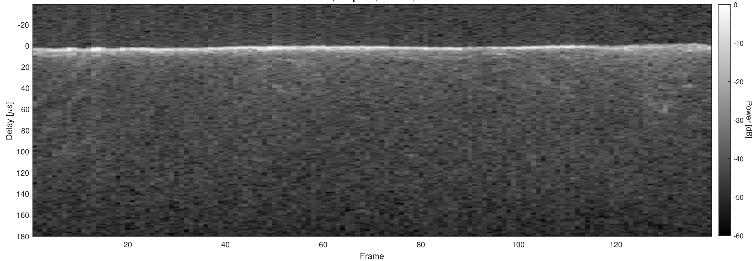
Orbit 15335, Chapman, Window, Channel 2
