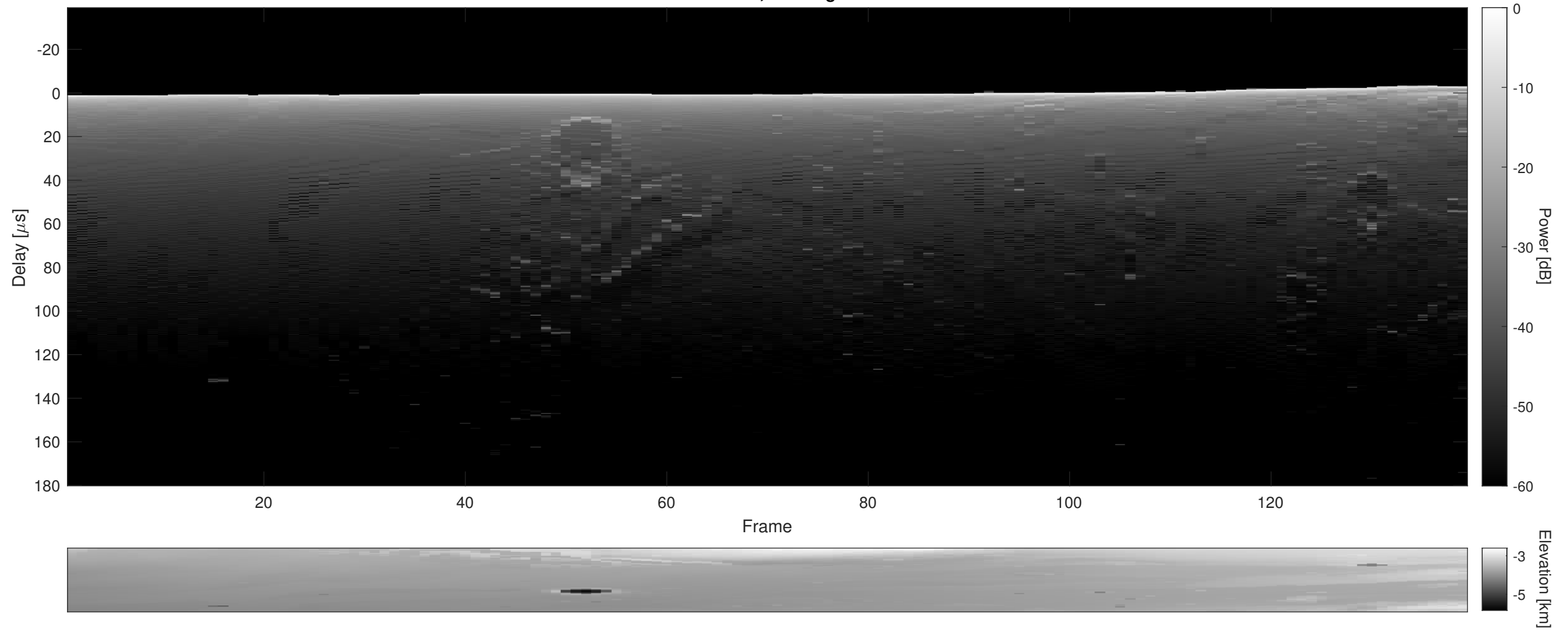
Orbit 15335, Cluttergram
