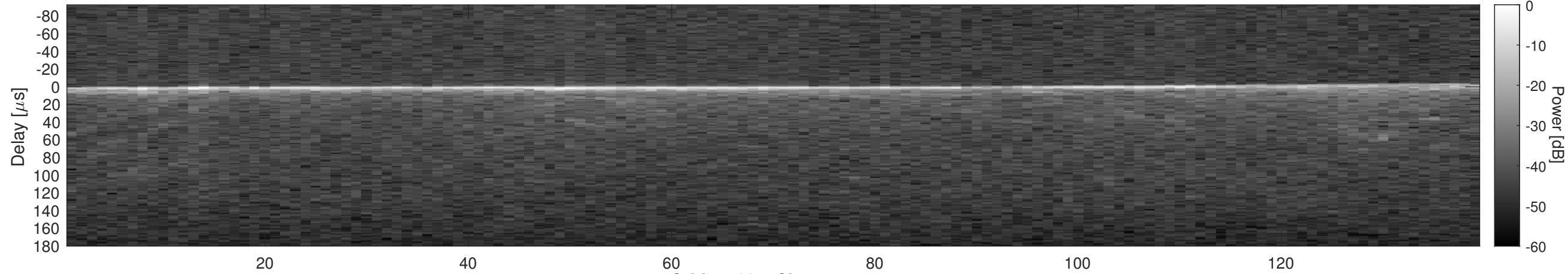
Orbit 15335, Cluttergram
