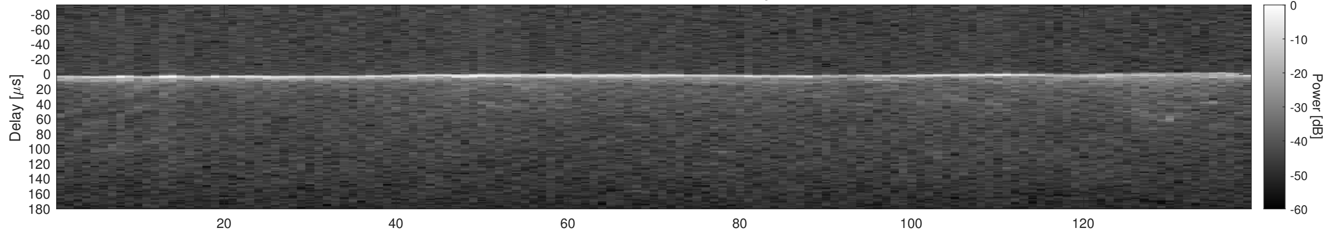
Orbit 15335, Window, Channel 1, Optimized
