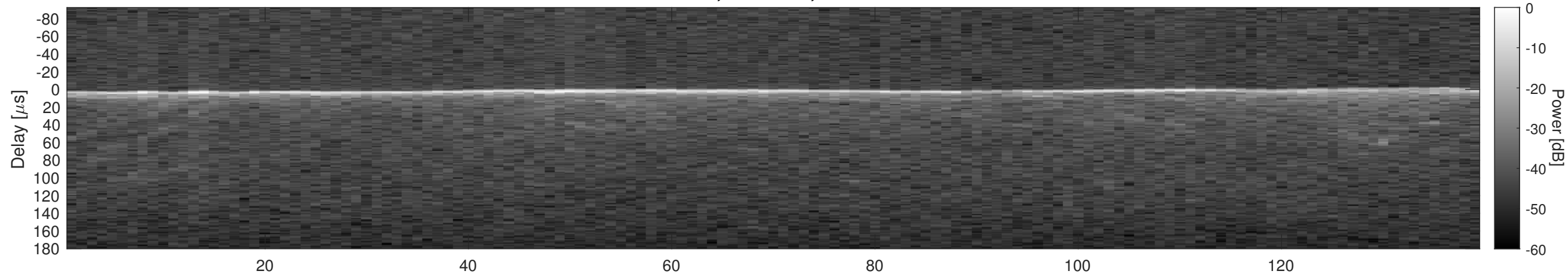
Orbit 15335, Window, Channel 1, Chapman
