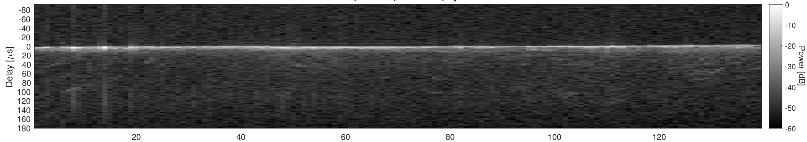
Orbit 15335, Cluttergram
