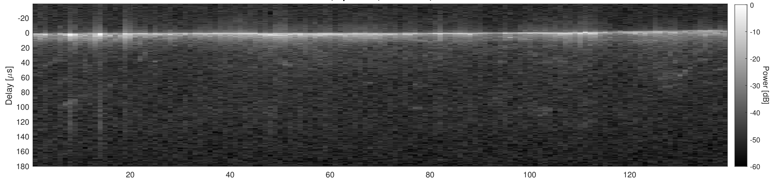
Orbit 15335, Cluttergram
