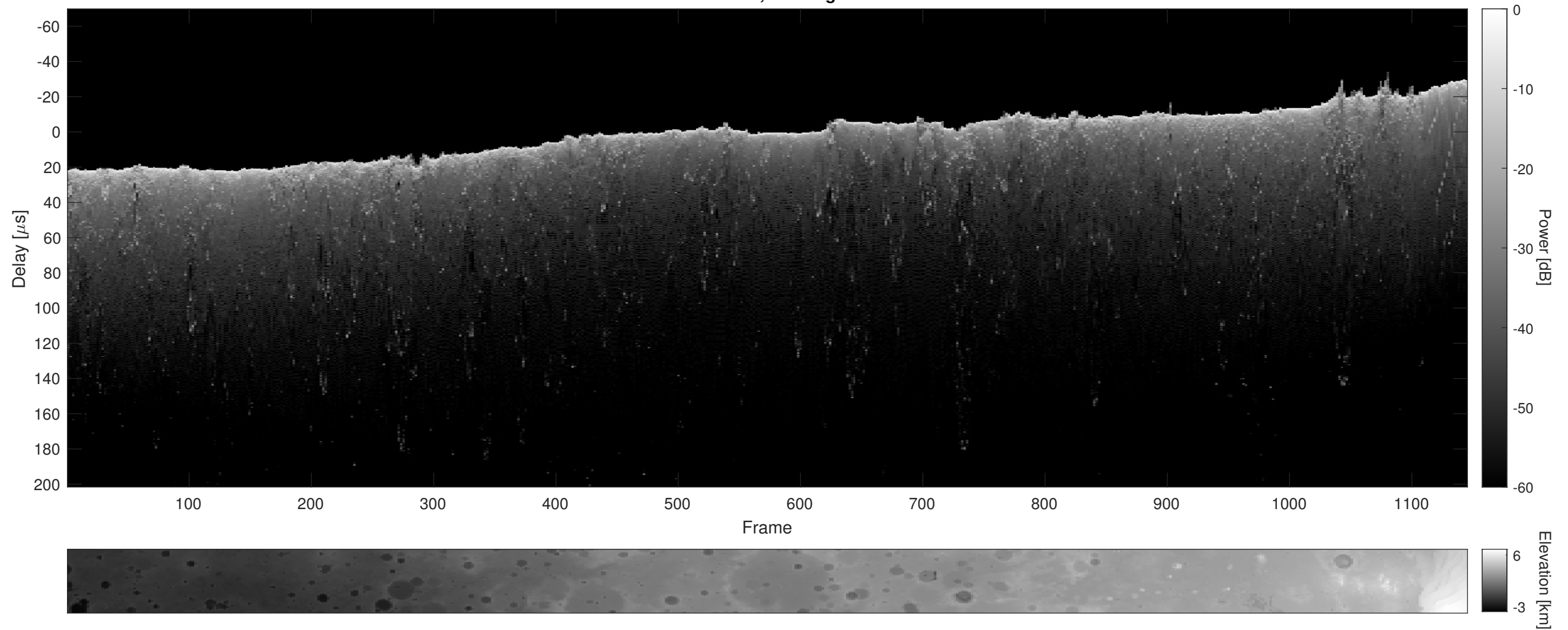
Orbit 15337, Cluttergram
