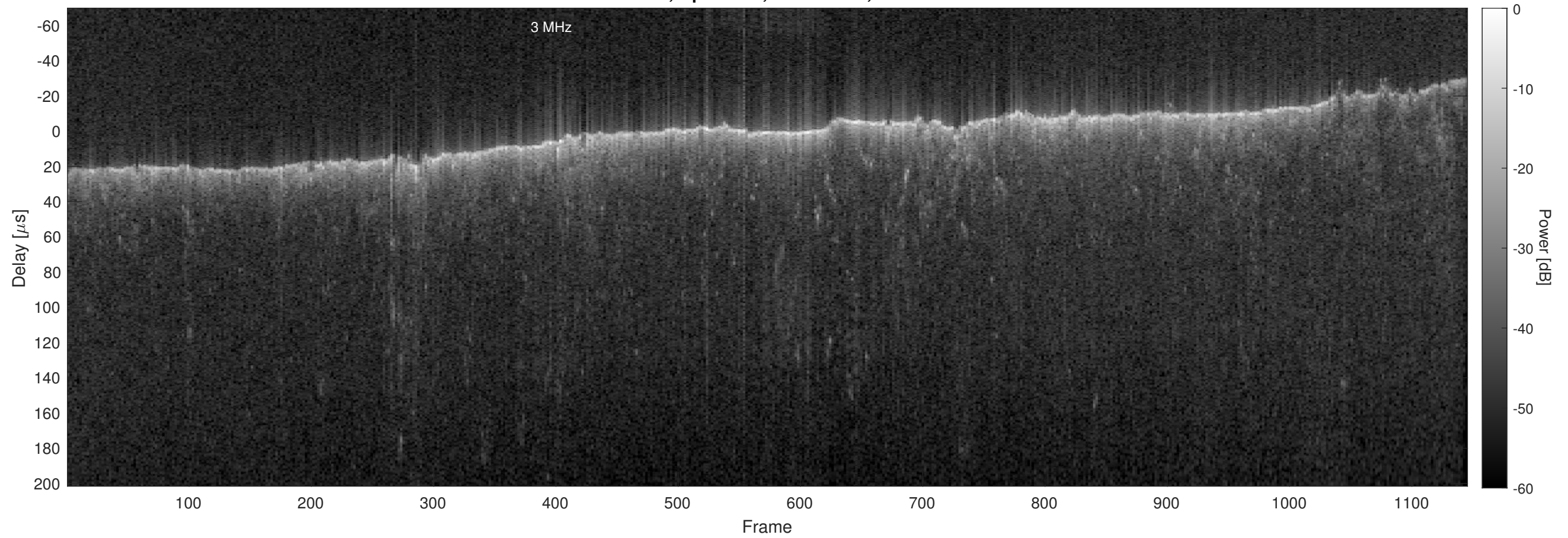
Orbit 15337, Optimized, No Window, Channel 2
