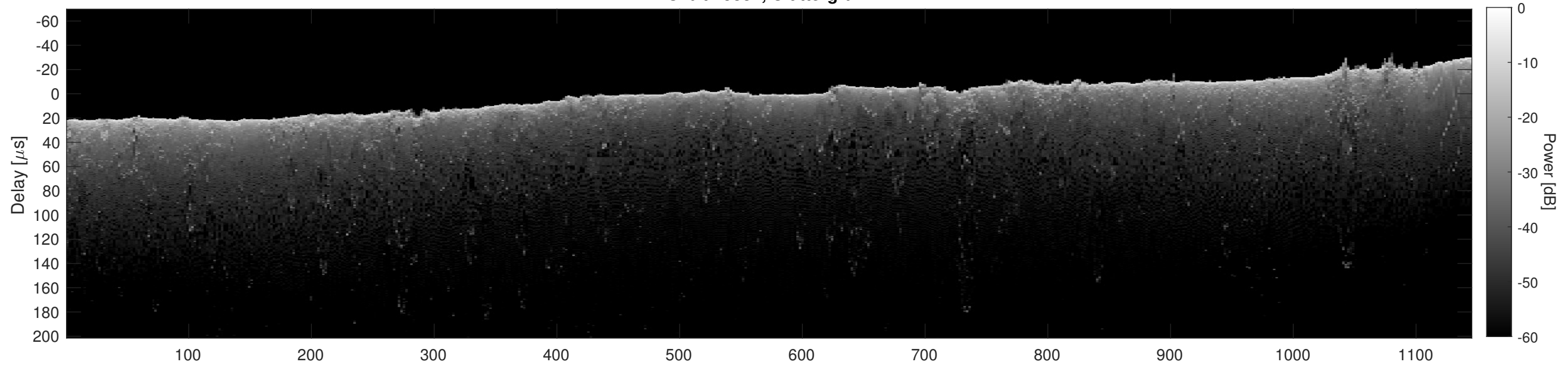
Orbit 15337, Cluttergram
