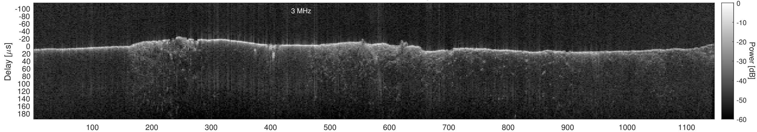
Orbit 15338, Cluttergram
