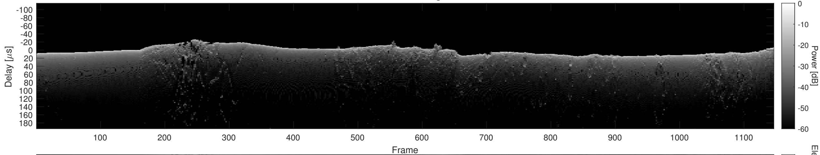
Orbit 15338, Cluttergram
