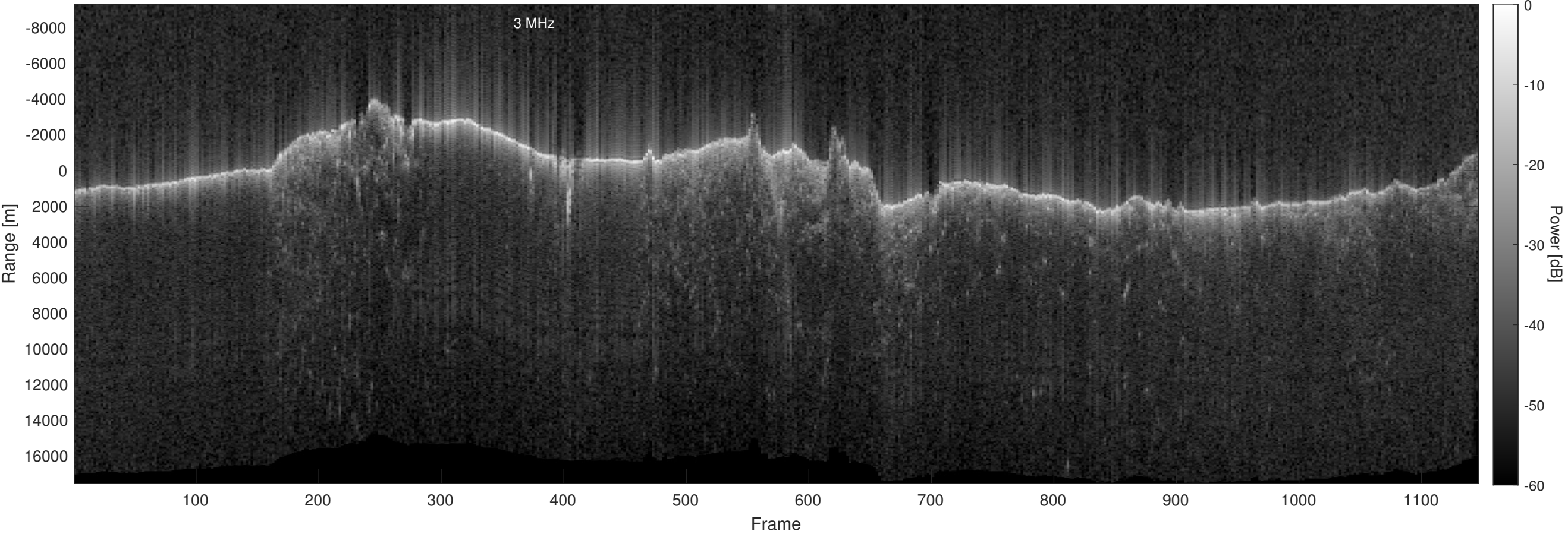
Orbit 15338, Optimized, No Window, Depth-Corrected, Channel 2
