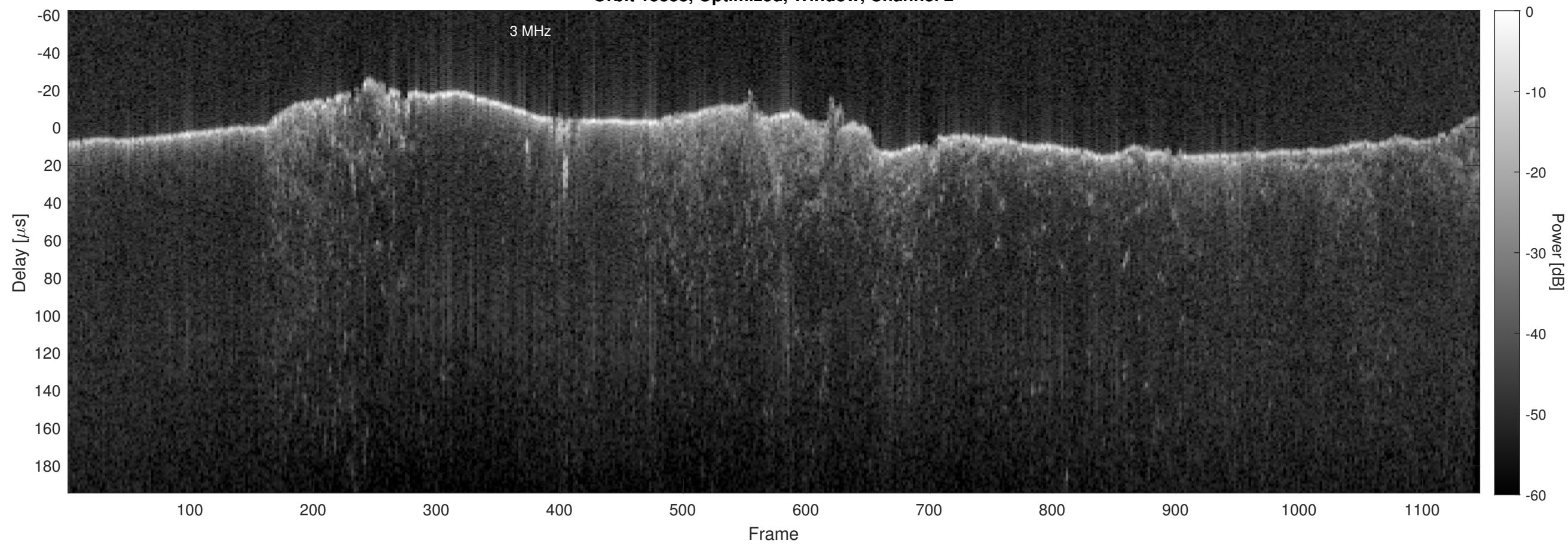
Orbit 15338, Optimized, Window, Channel 2
