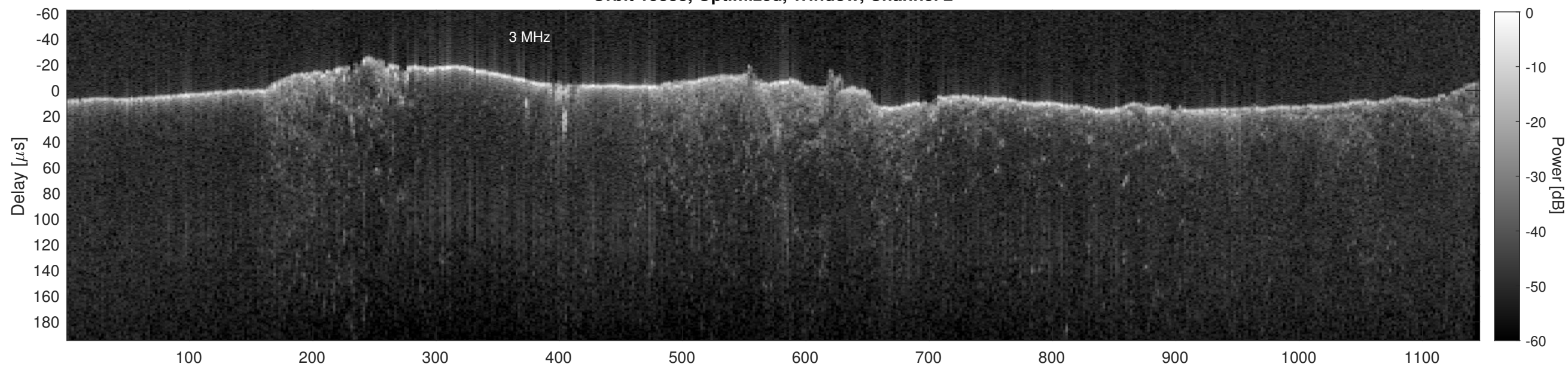
Orbit 15338, Cluttergram
