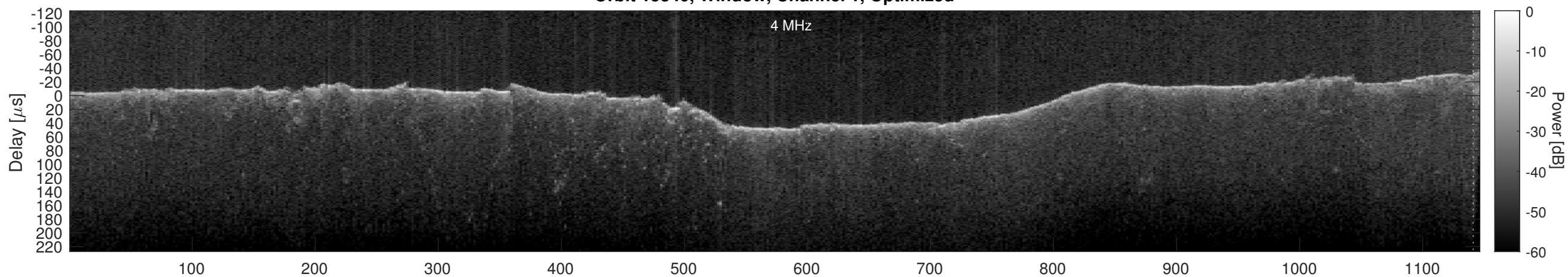
Orbit 15340, Cluttergram
