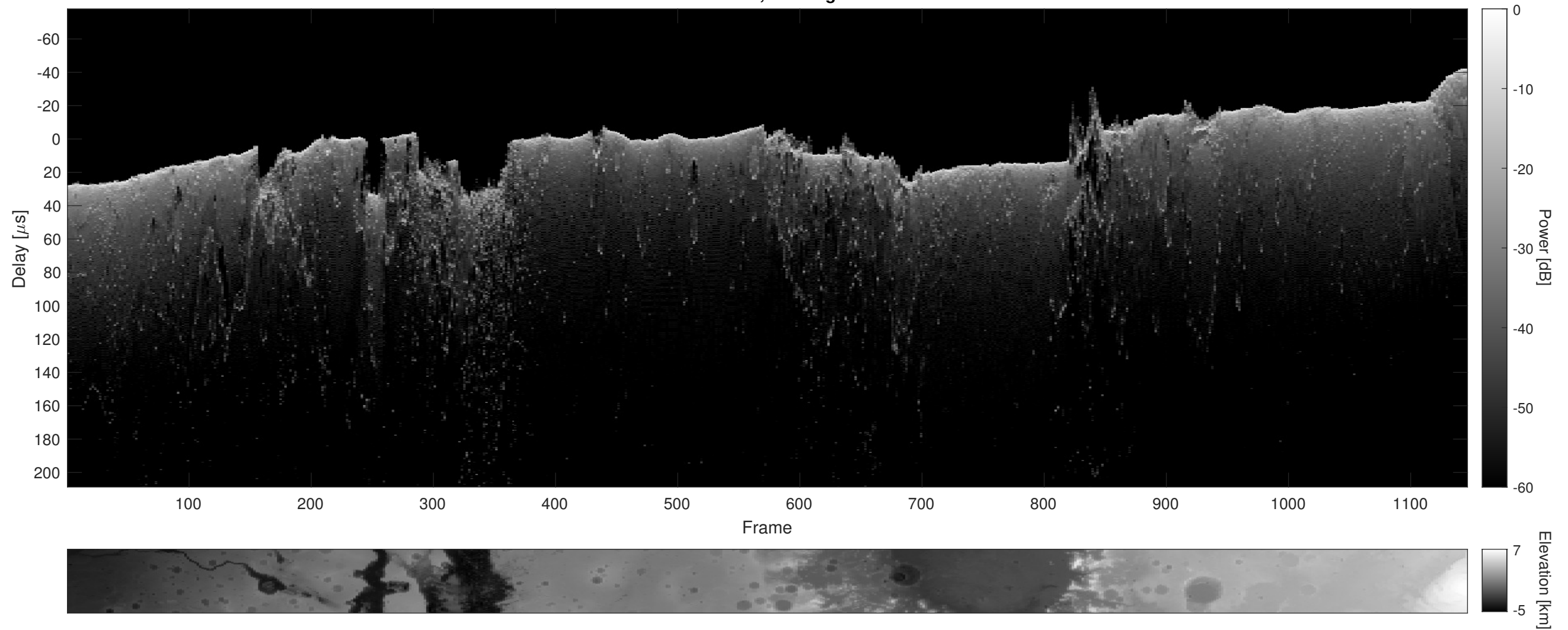
Orbit 15341, Cluttergram
