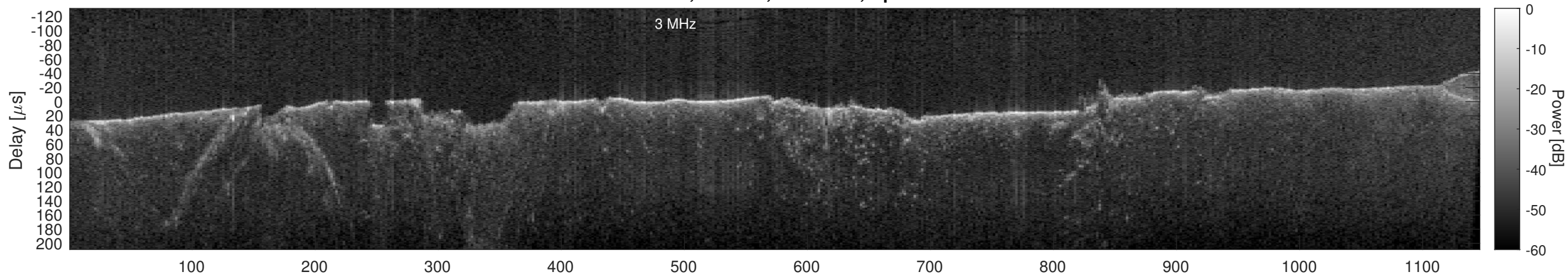
Orbit 15341, Cluttergram
