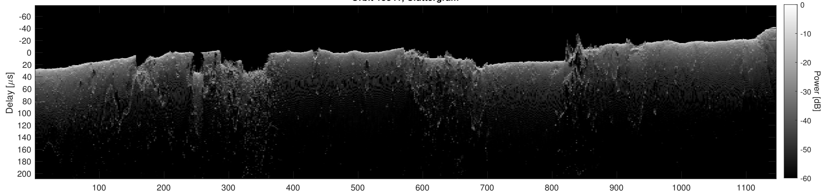
Orbit 15341, Cluttergram
