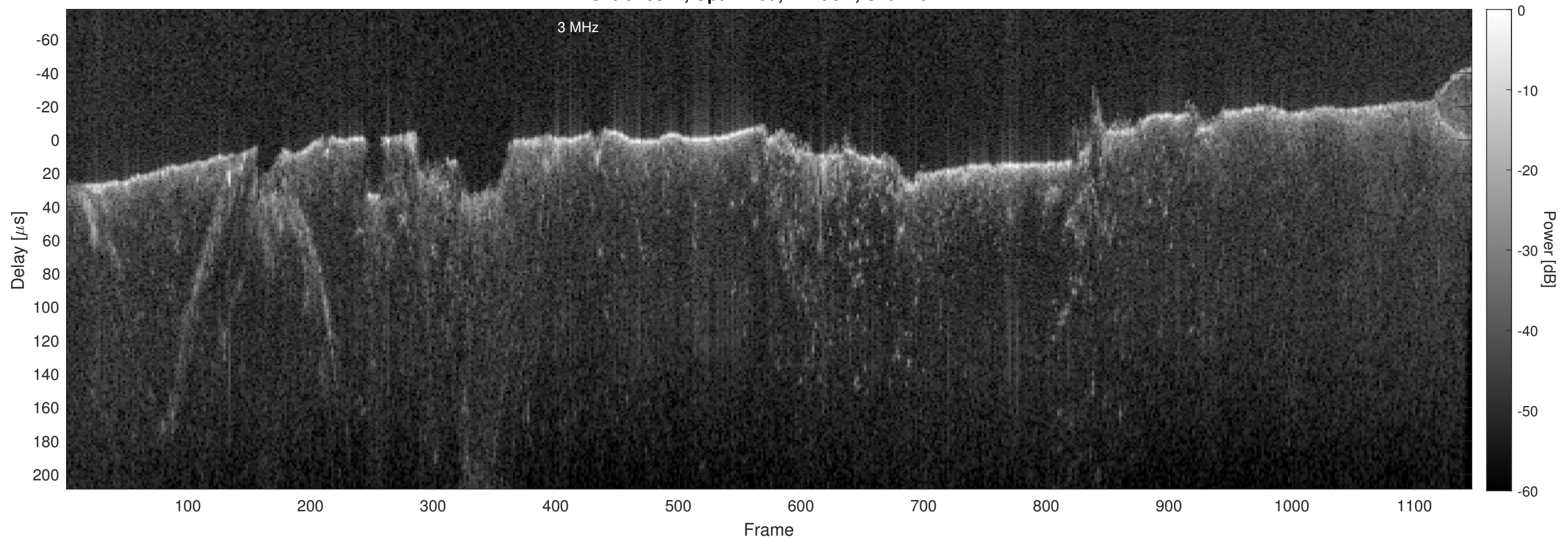
Orbit 15341, Optimized, Window, Channel 2
