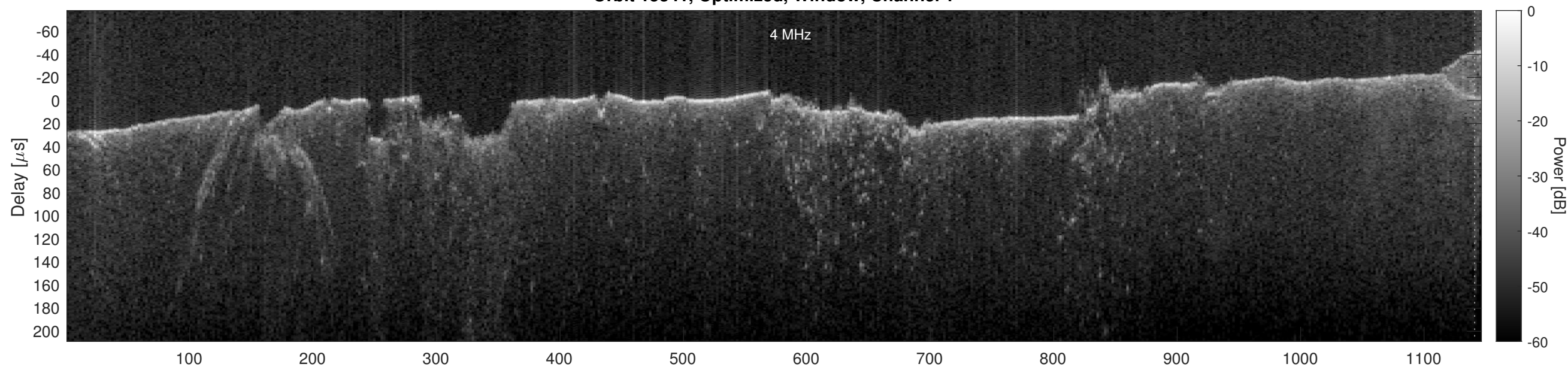
Orbit 15341, Optimized, Window, Channel 2
