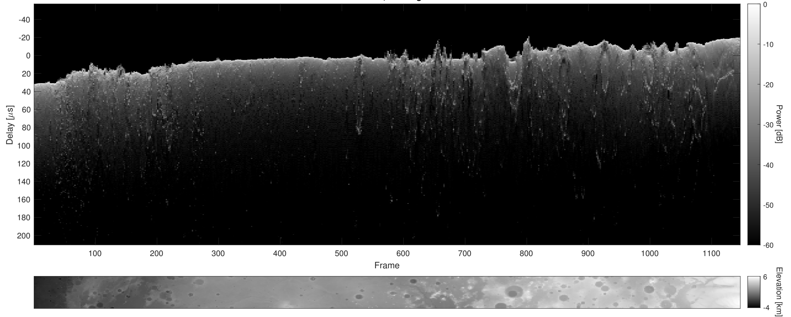
Orbit 15343, Cluttergram
