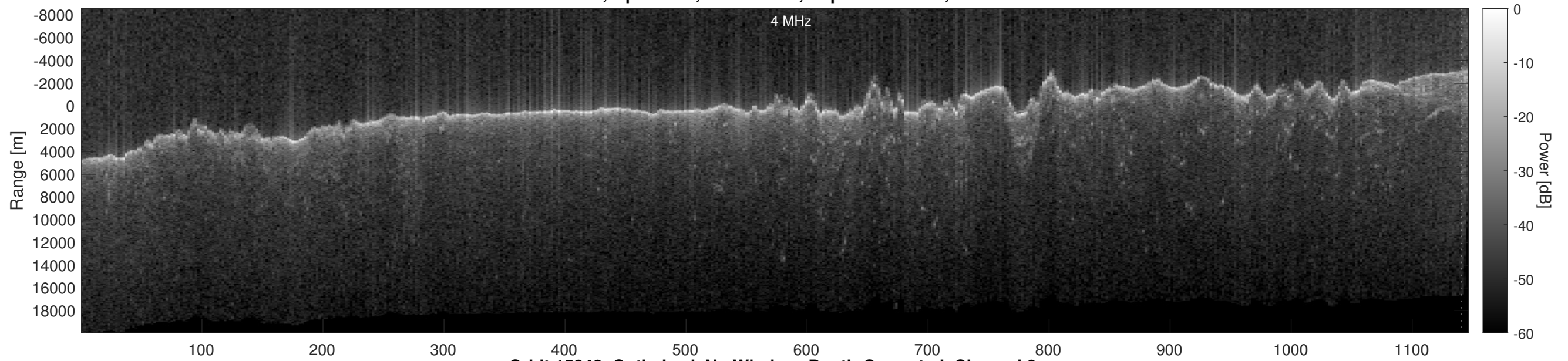
Orbit 15343, Optimized, No Window, Depth-Corrected, Channel 2
