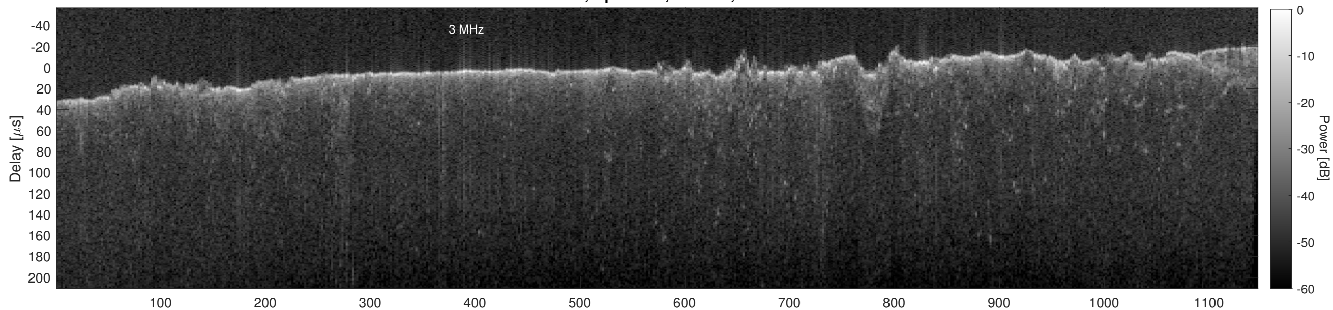
Orbit 15343, Cluttergram
