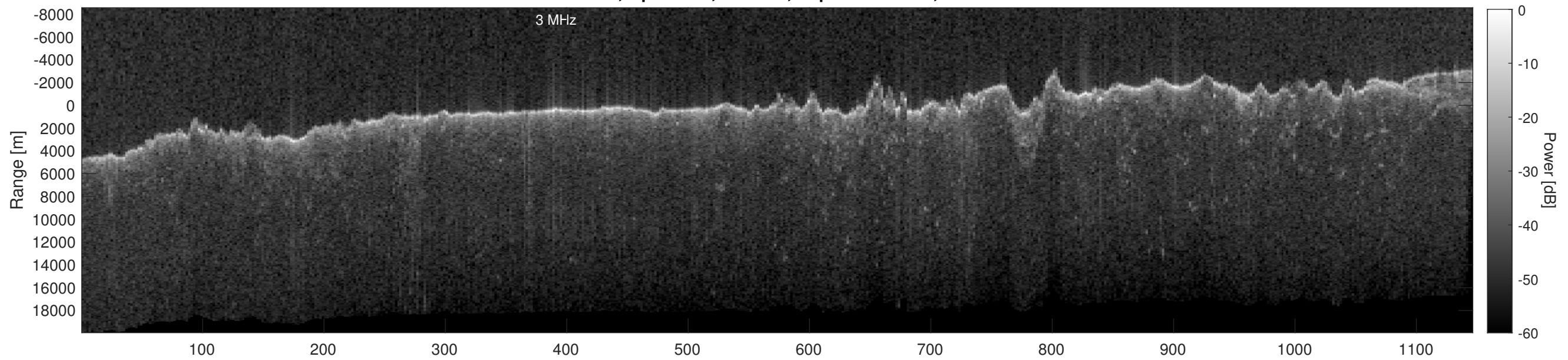
Orbit 15343, Depth-Corrected Cluttergram
