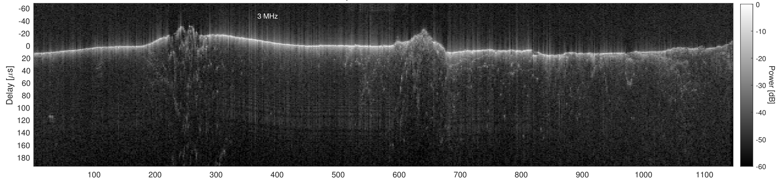
Orbit 15345, Cluttergram
