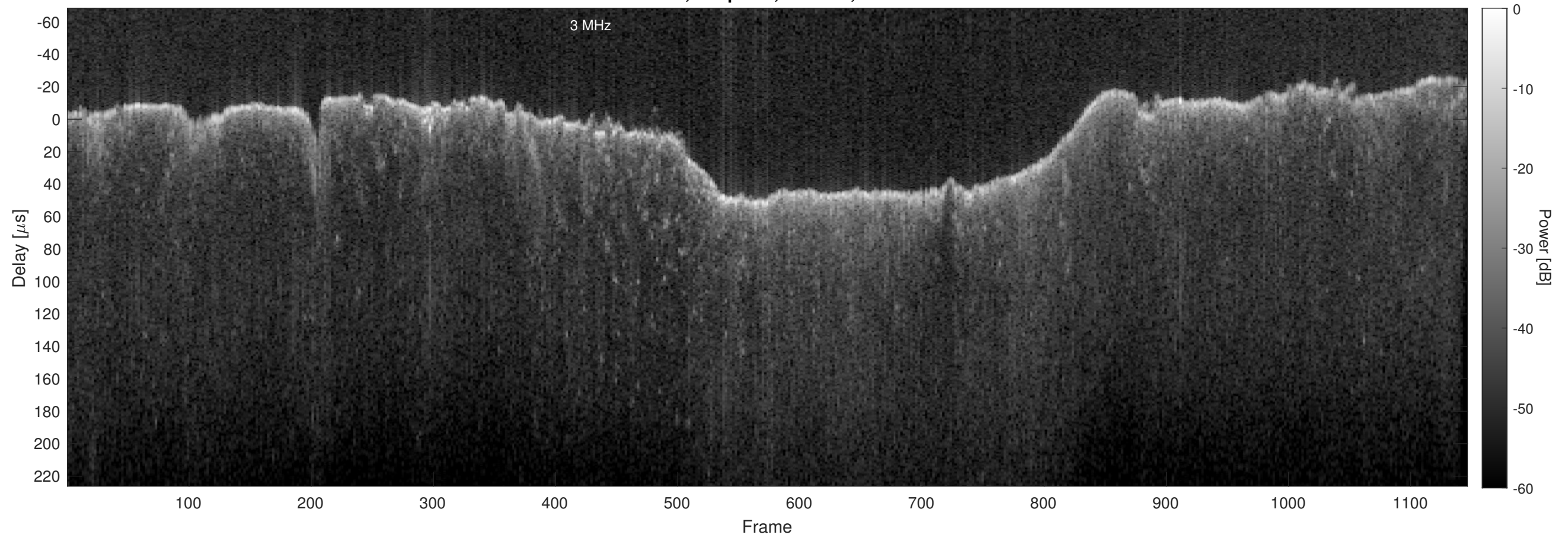
Orbit 15347, Chapman, Window, Channel 2
