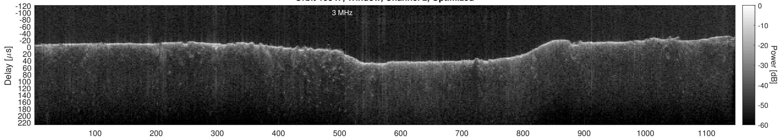
Orbit 15347, Cluttergram
