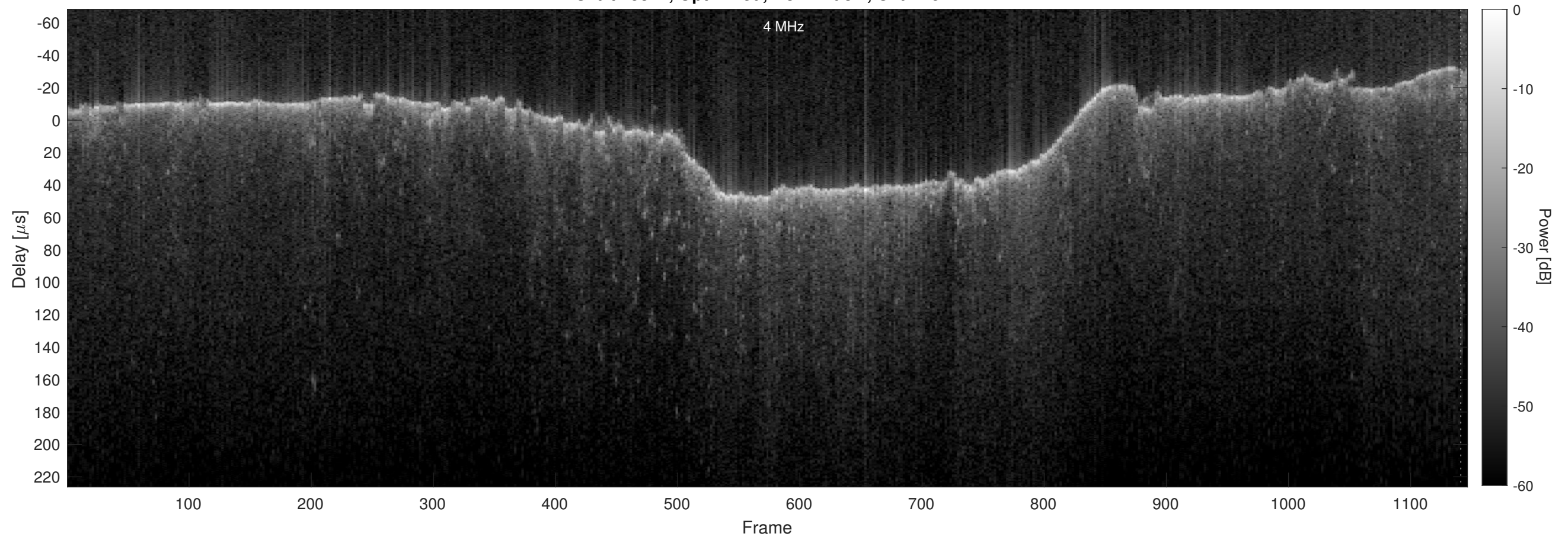
Orbit 15347, Optimized, No Window, Channel 2
