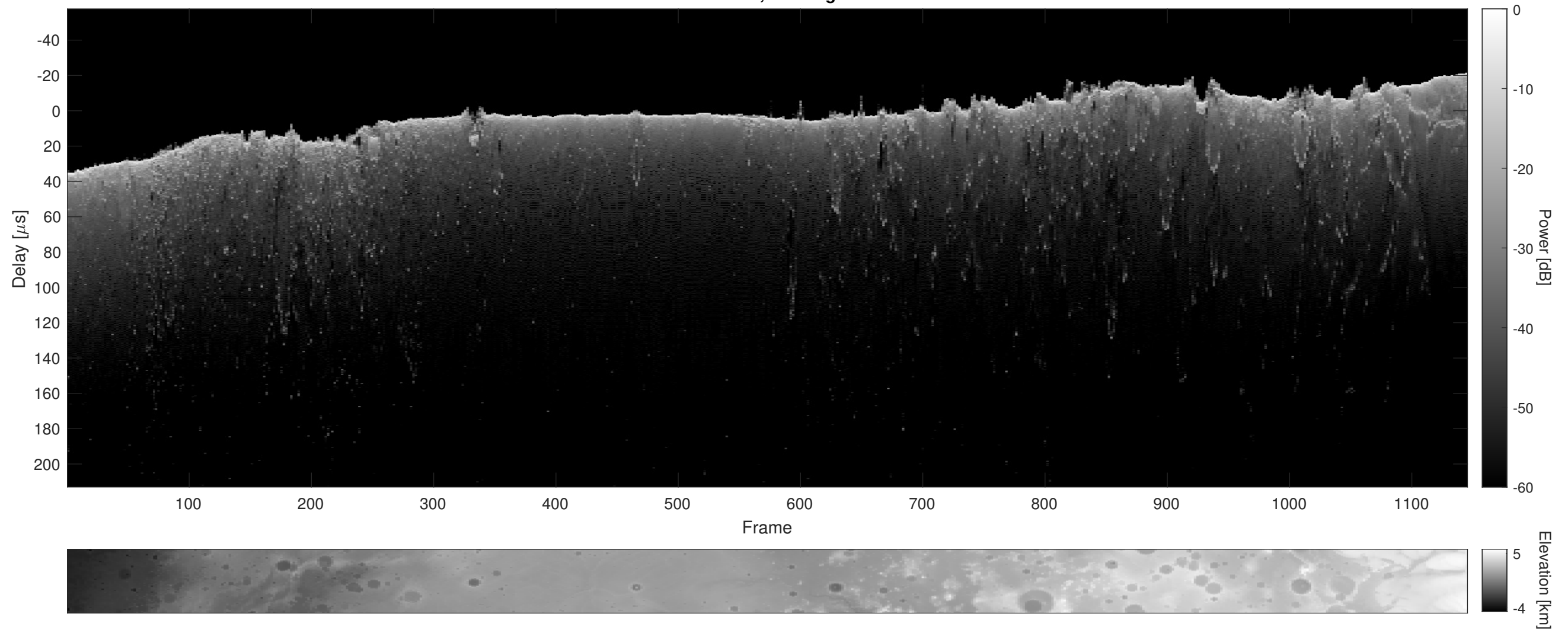
Orbit 15350, Cluttergram
