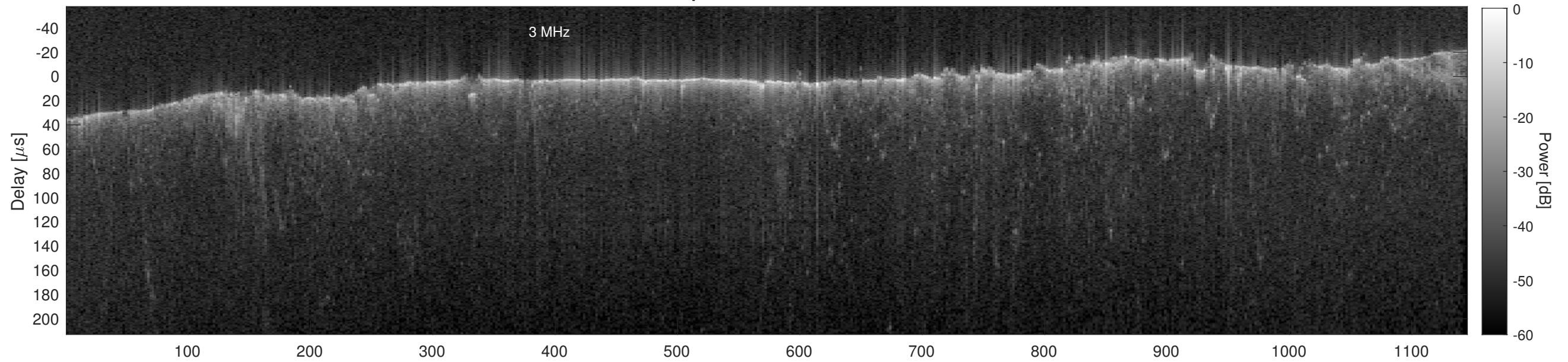
Orbit 15350, Cluttergram
