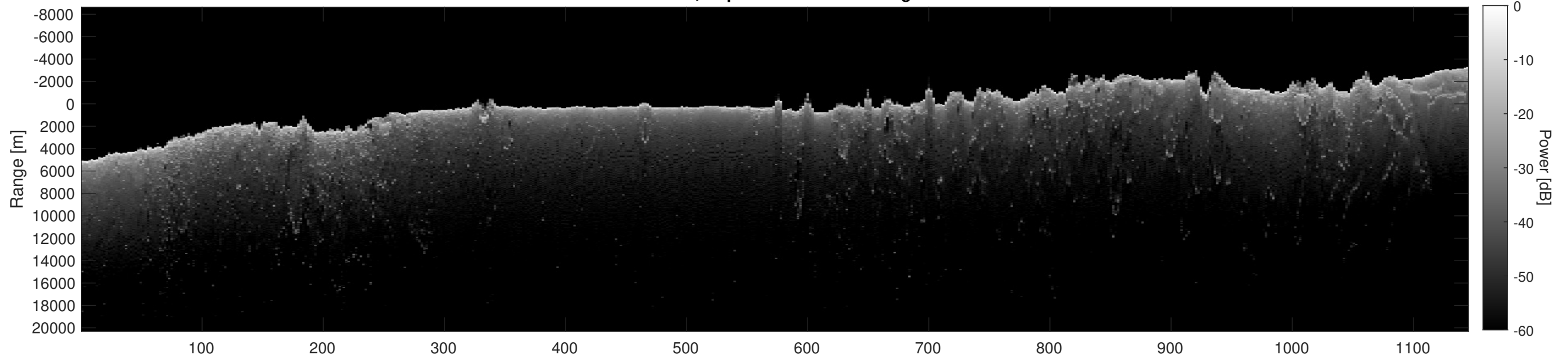
Orbit 15350, Depth-Corrected Cluttergram
