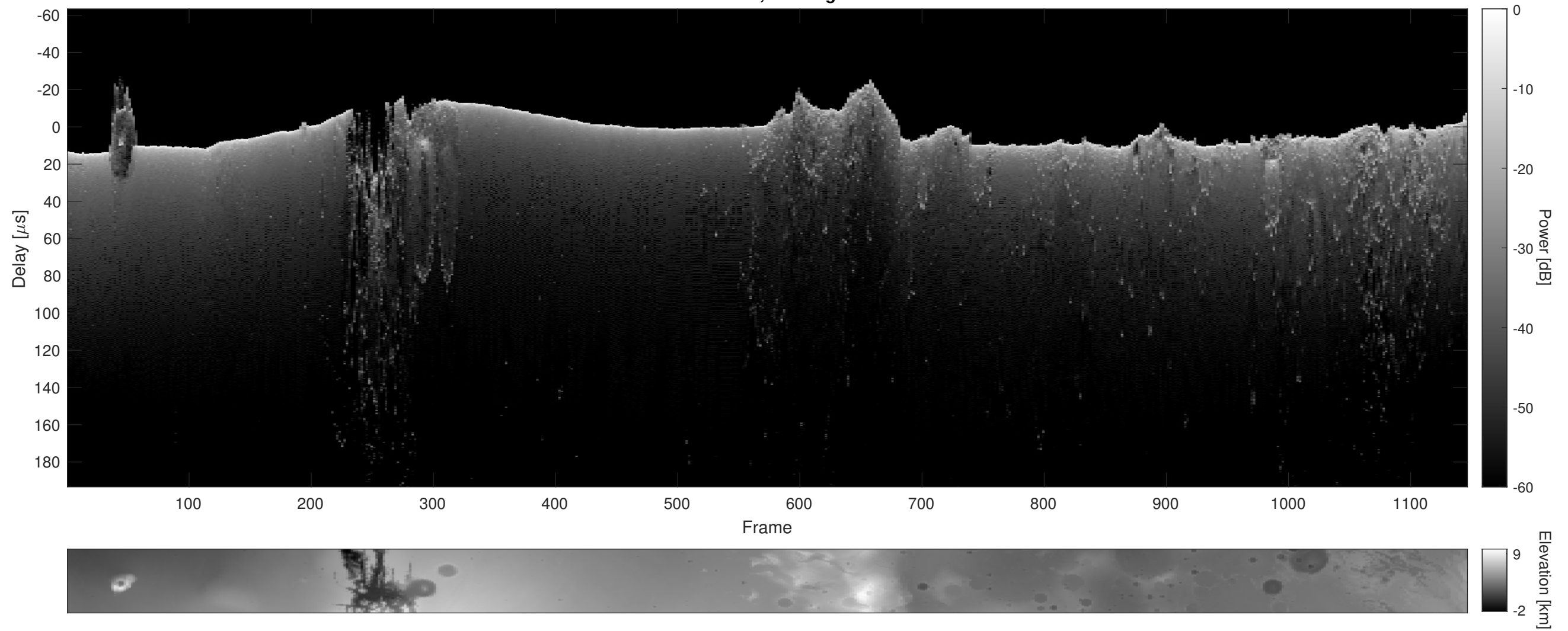
Orbit 15352, Cluttergram
