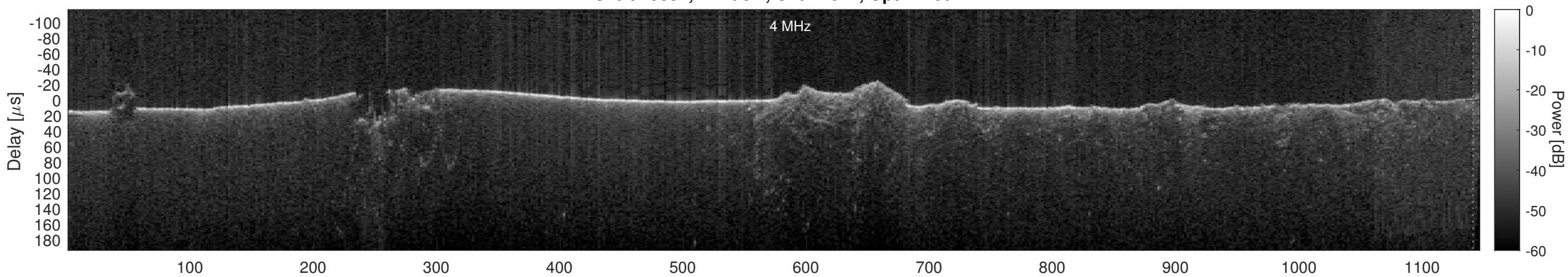
Orbit 15352, Cluttergram
