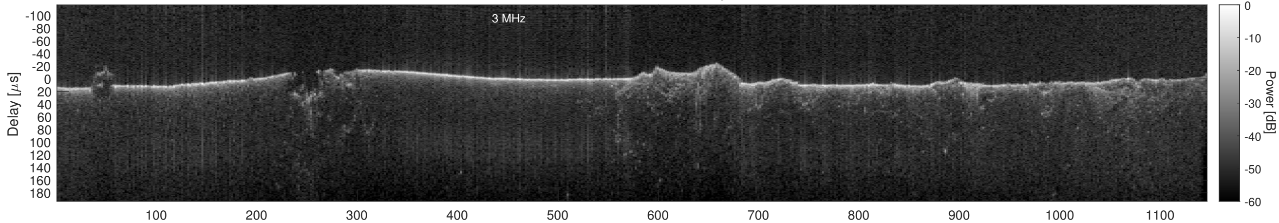
Orbit 15352, Cluttergram
