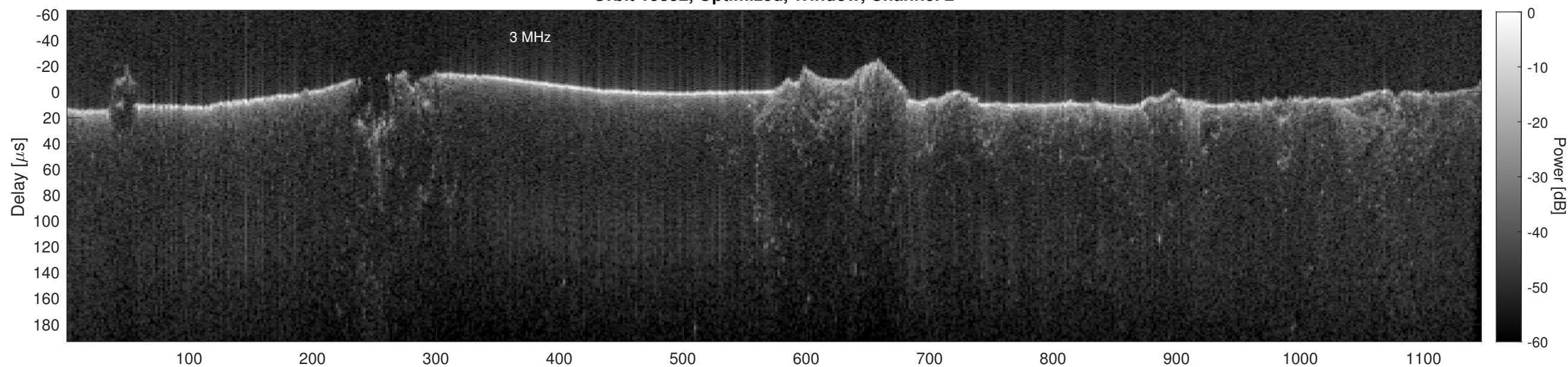
Orbit 15352, Cluttergram
