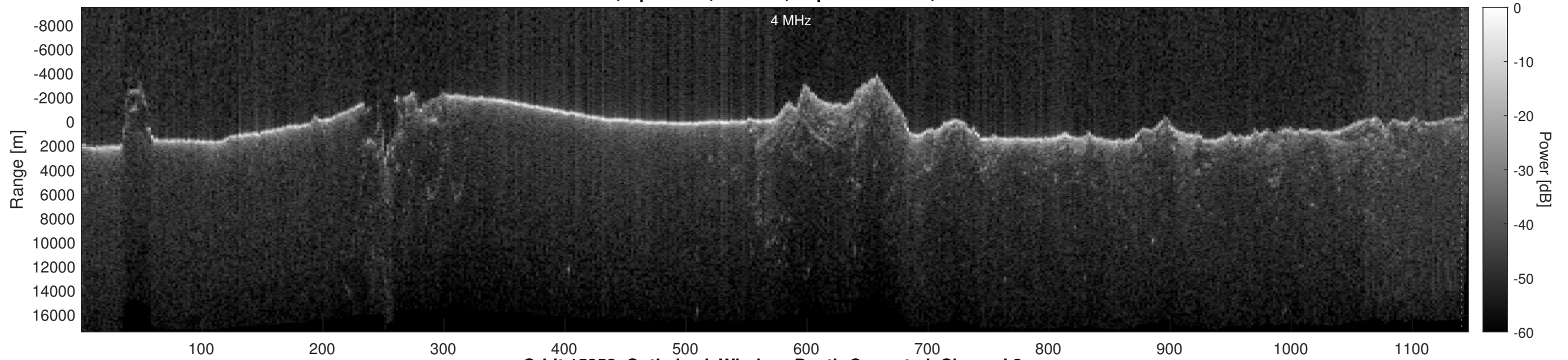
Orbit 15352, Optimized, Window, Depth-Corrected, Channel 2
