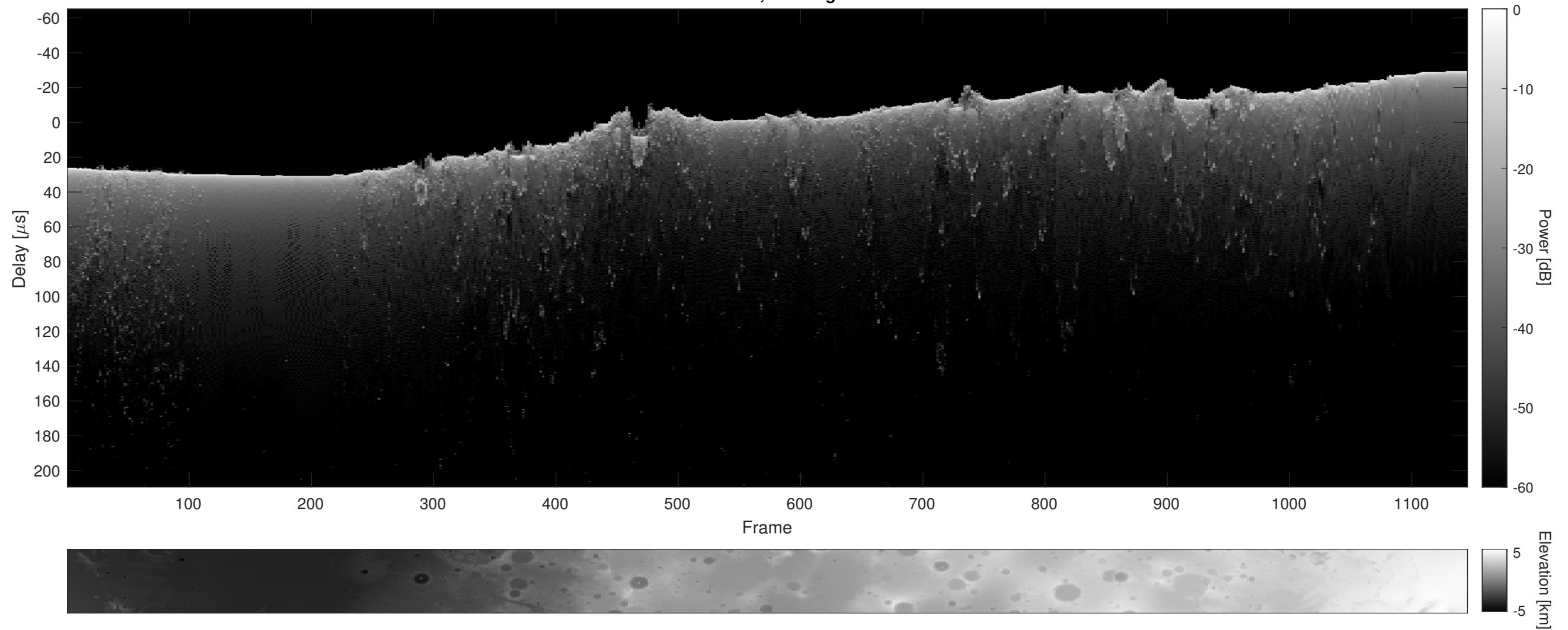
Orbit 15353, Cluttergram
