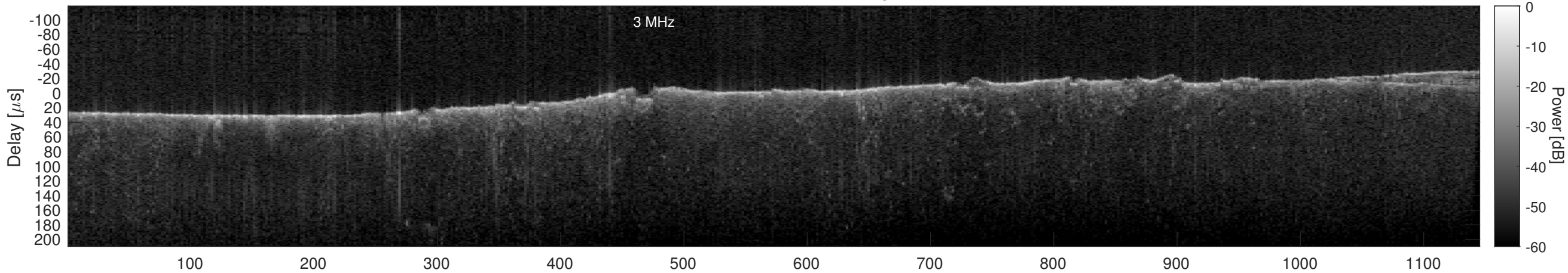
Orbit 15353, Cluttergram
