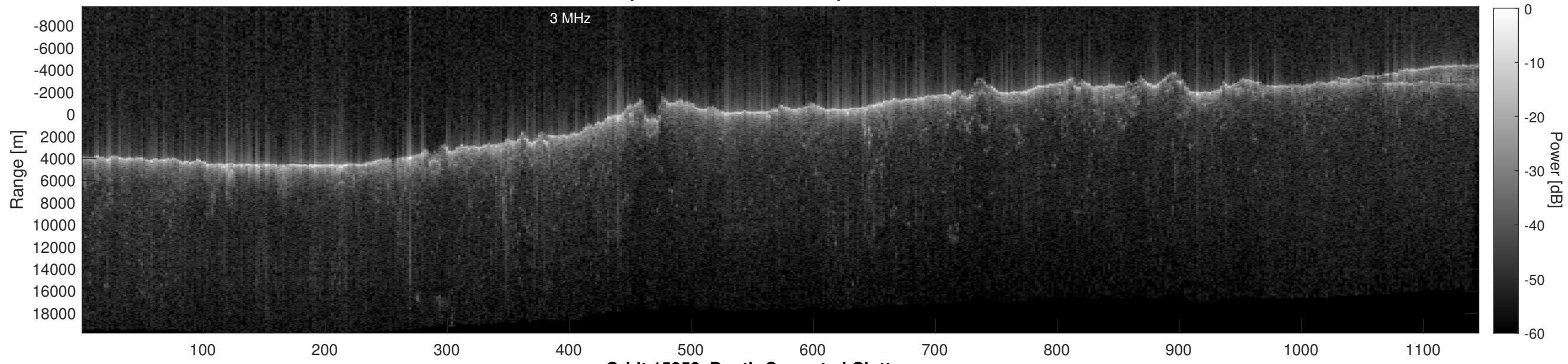
Orbit 15353, Depth-Corrected Cluttergram
