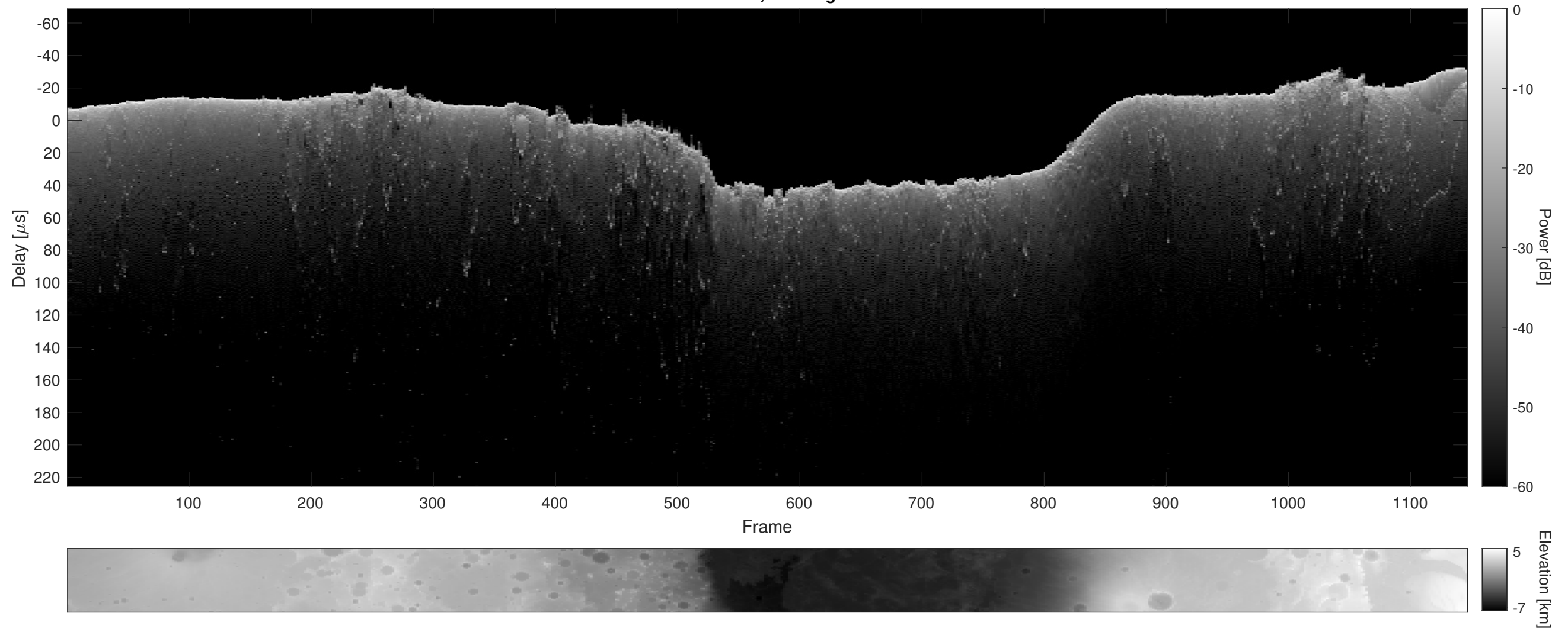
Orbit 15354, Cluttergram
