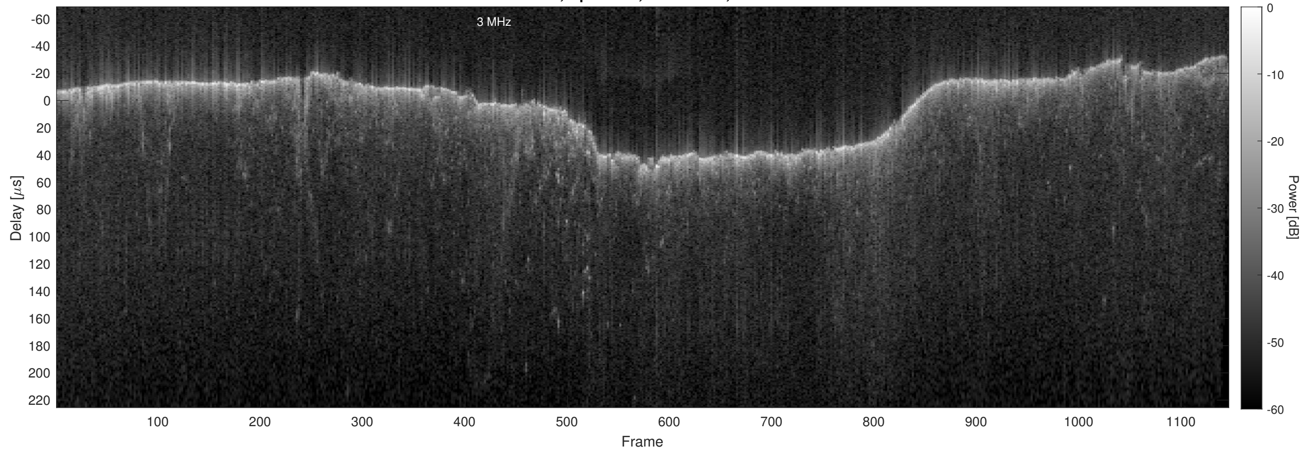
Orbit 15354, Optimized, No Window, Channel 2
