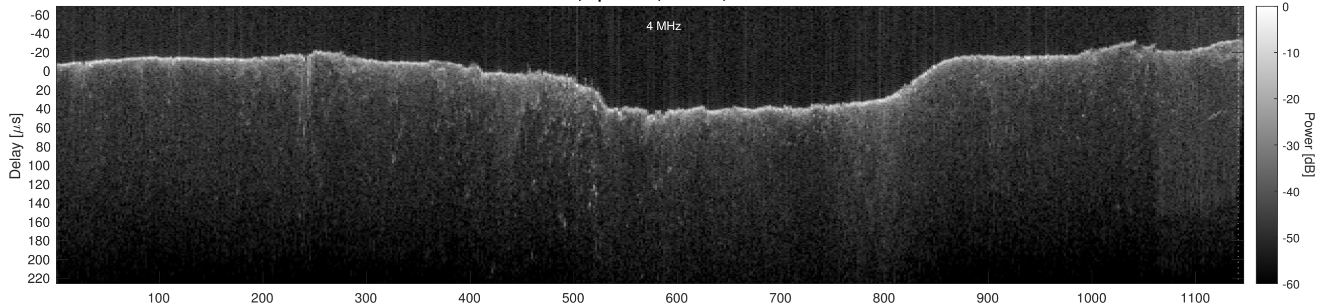
Orbit 15354, Optimized, Window, Channel 2
