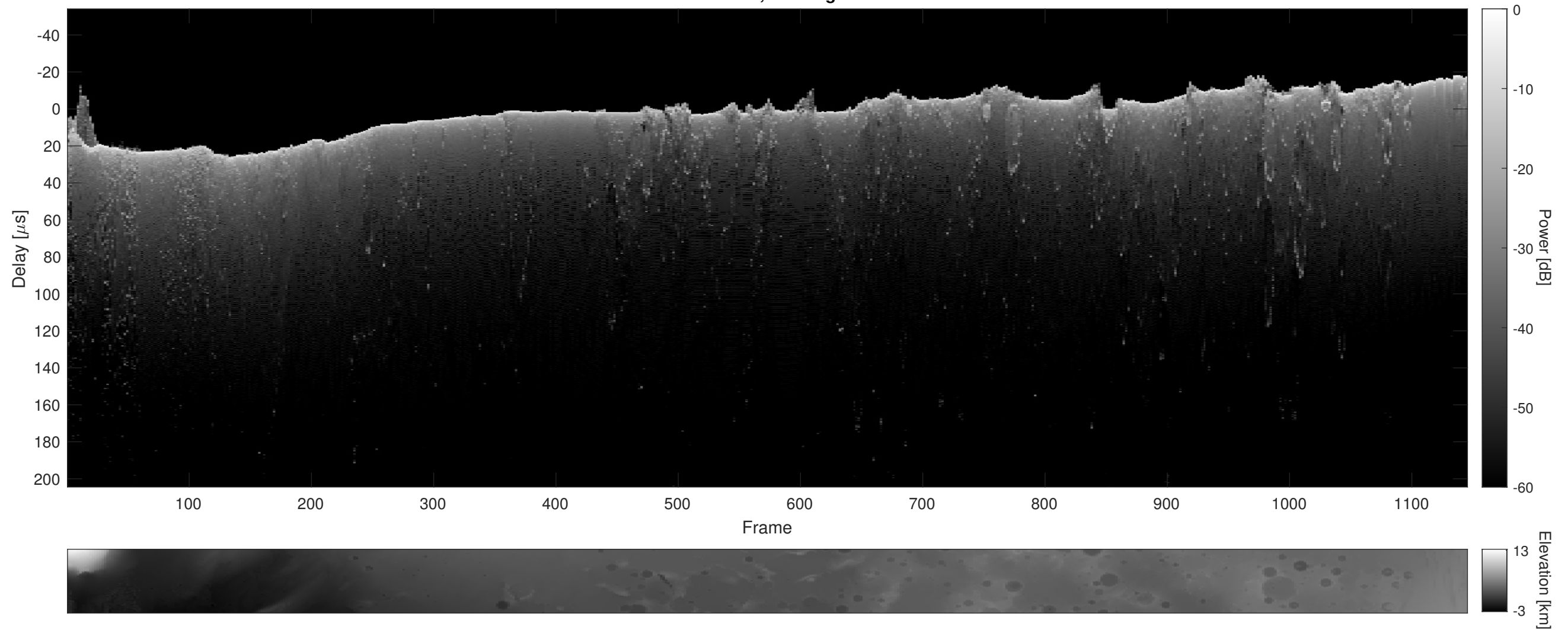
Orbit 15356, Cluttergram
