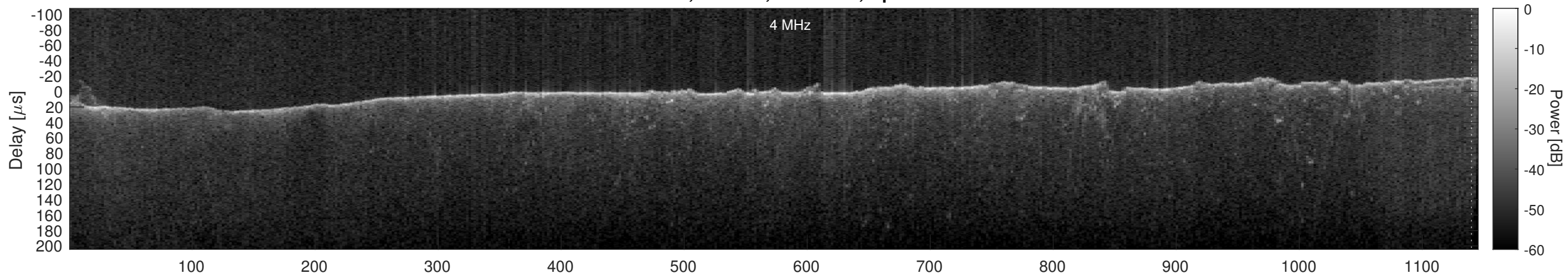
Orbit 15356, Cluttergram
