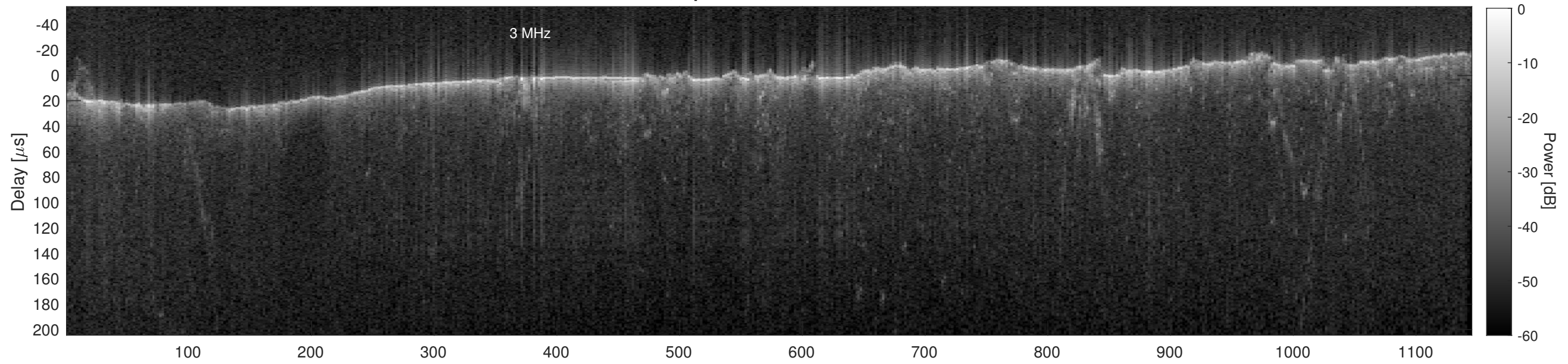
Orbit 15356, Cluttergram
