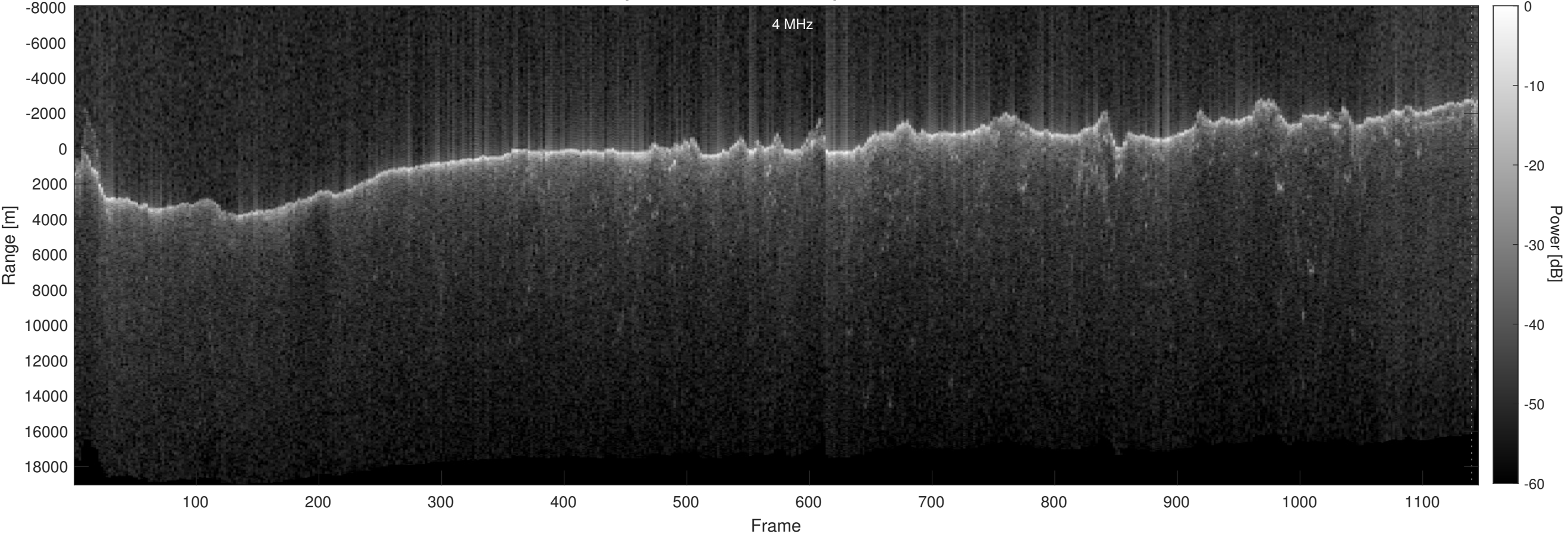
Orbit 15356, Optimized, No Window, Depth-Corrected, Channel 2
