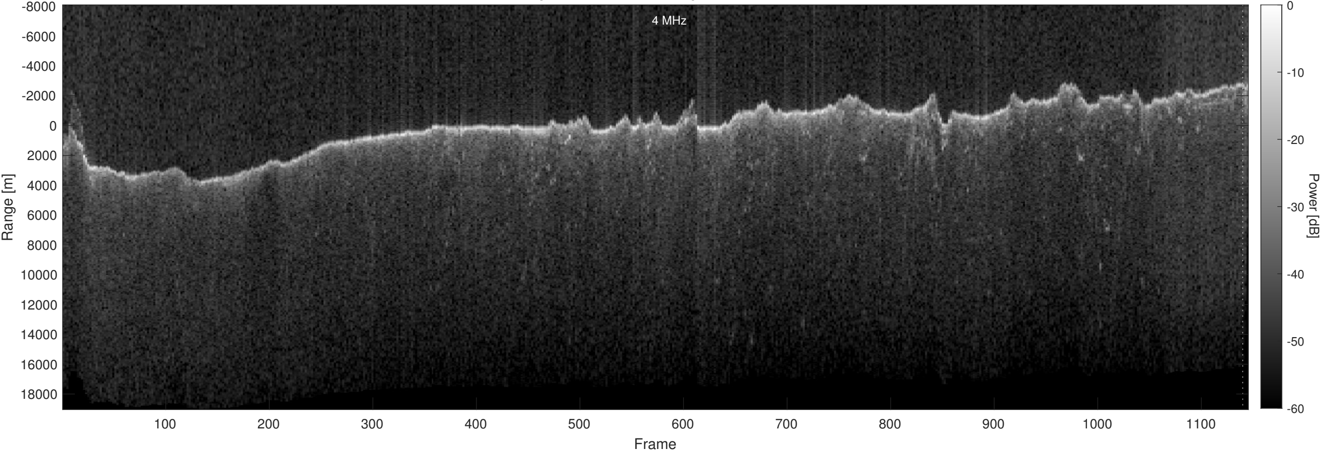
Orbit 15356, Optimized, Window, Depth-Corrected, Channel 2
