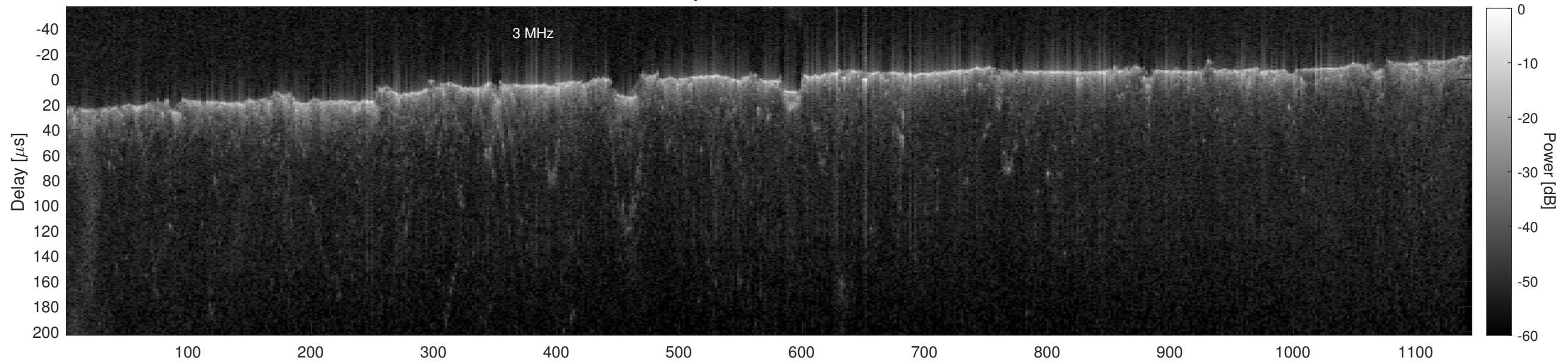
Orbit 15358, Cluttergram
