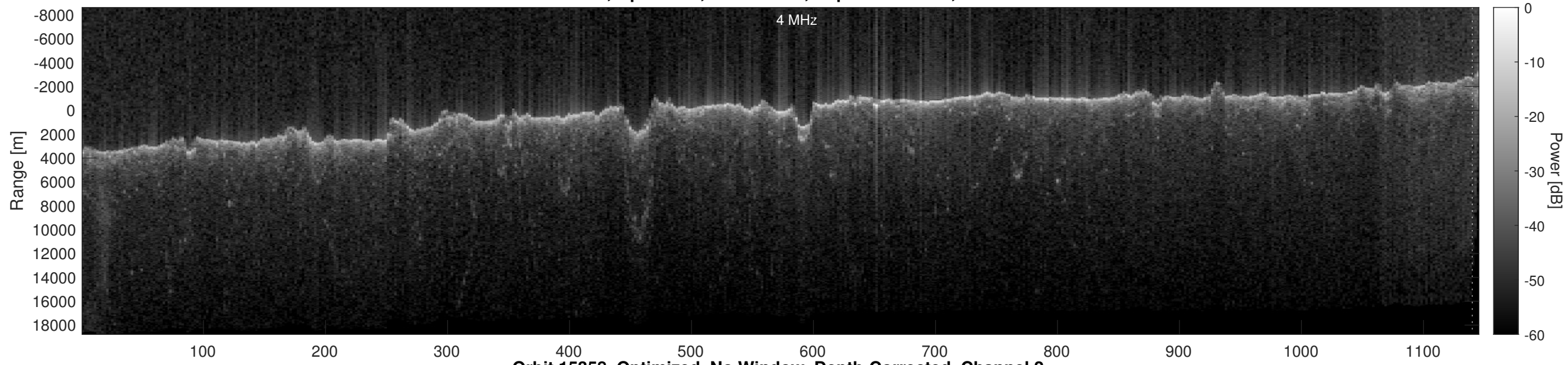
Orbit 15358, Optimized, No Window, Depth-Corrected, Channel 2
