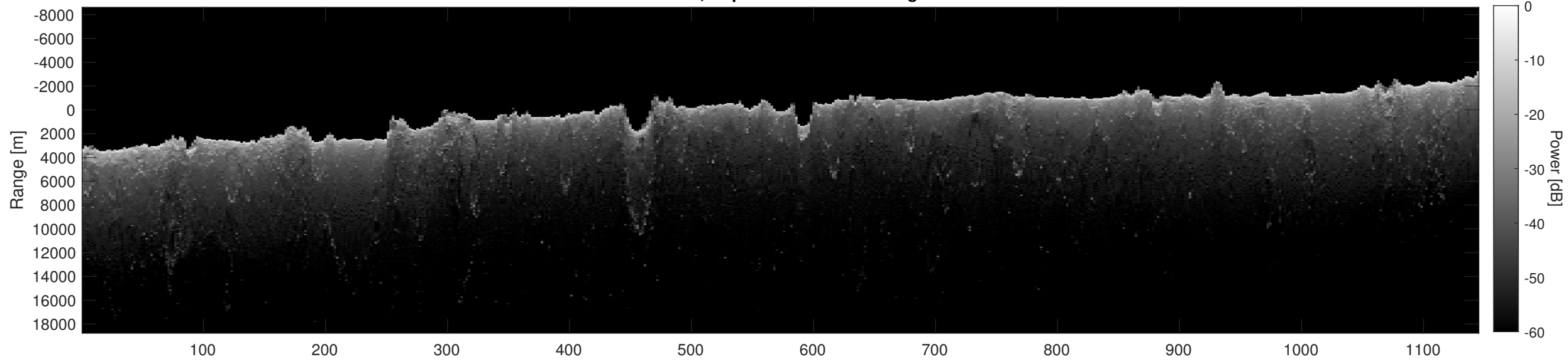
Orbit 15358, Depth-Corrected Cluttergram
